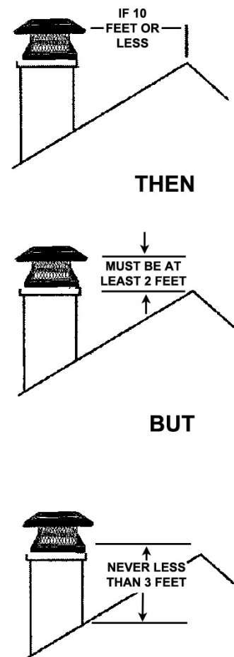
Figure 25. Chimney Height
