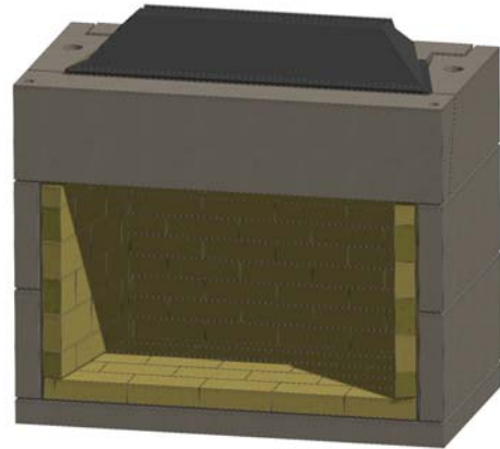
Figure 12. Damper Placement
