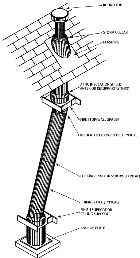
Figure 26. Metal Chimney Construction
