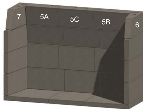
Figure 8. Upper Back Plates & Sidewalls
