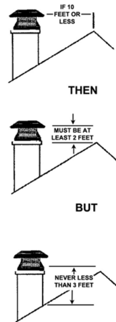
Figure 27. Chimney Height
