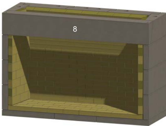
Figure 11. Front Lintel
