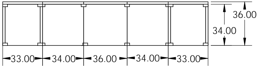
End View
