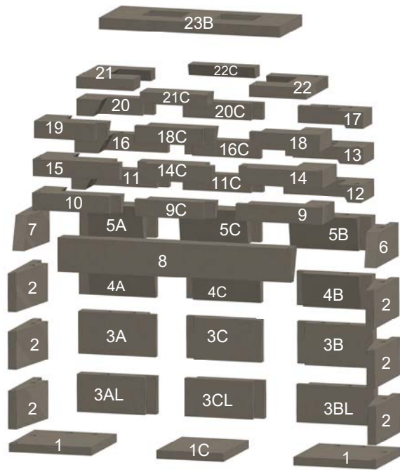
Figure 2. Fireplace Components
