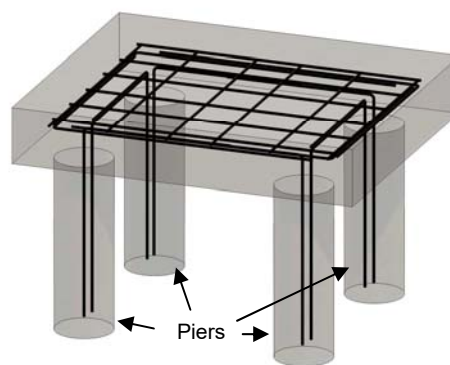
Figure 4. Footing with Piers - Cutaway View
