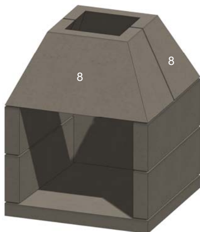
Figure 12. Throat Pieces
