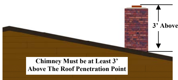
Figure 27. Chimney Height
