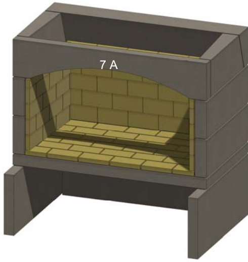
Figure 20. Front Lintel
