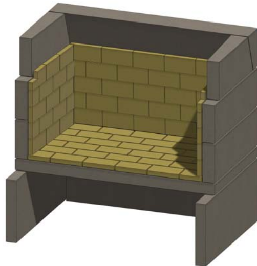
Figure 19. Sidewall Firebrick
