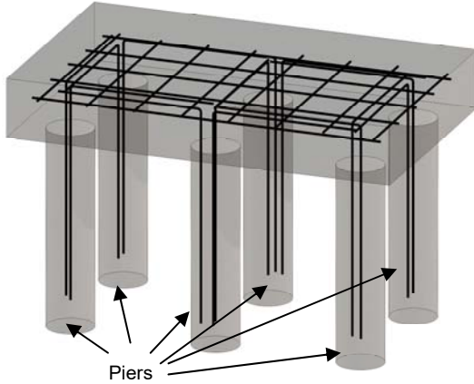
Figure 4. Footing with Piers - Cutaway View
