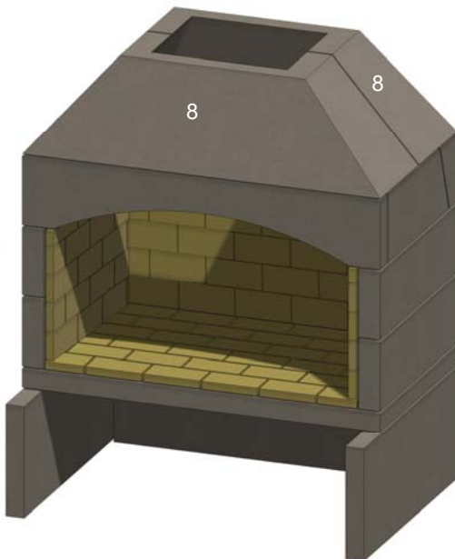
Figure 21. Throat Pieces
