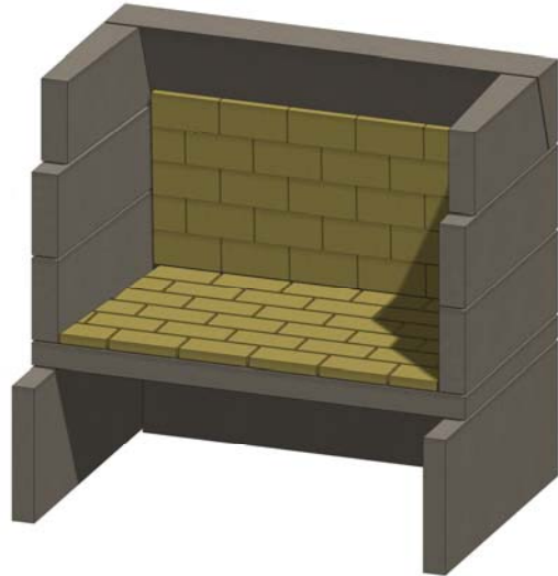
Figure 18. Back Wall Firebrick
