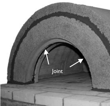
Figure J Fill joint between Liner Shell and Front Wall
