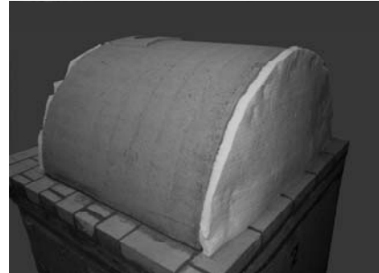
Figure F Glue blanket to rear wall
