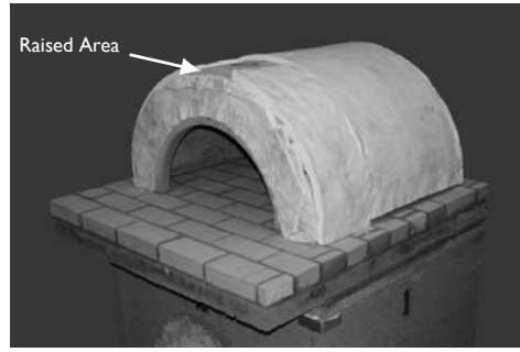
Figure H Fit blanket over Liner Shell, do not cover raised area
