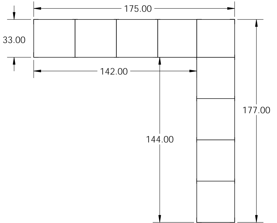
End View
